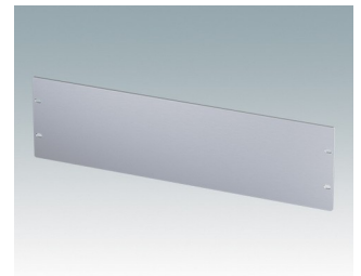
M6019001 Frontplatte 3HEX19" Aluminium Matt eloxiert 482,6x3x132,5mm
